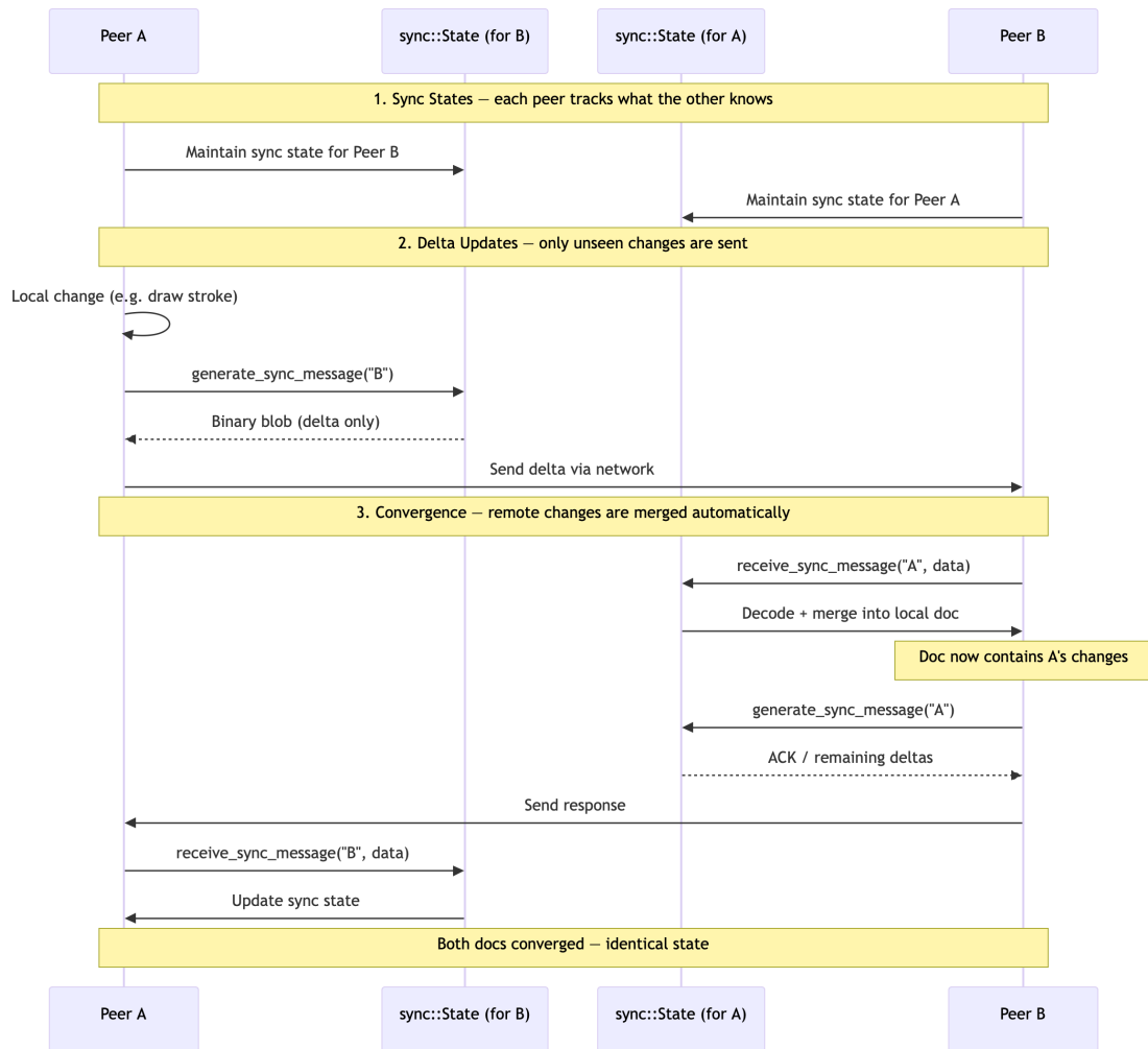
Figure 2.5: Automerger synchronization sequence between two peers
