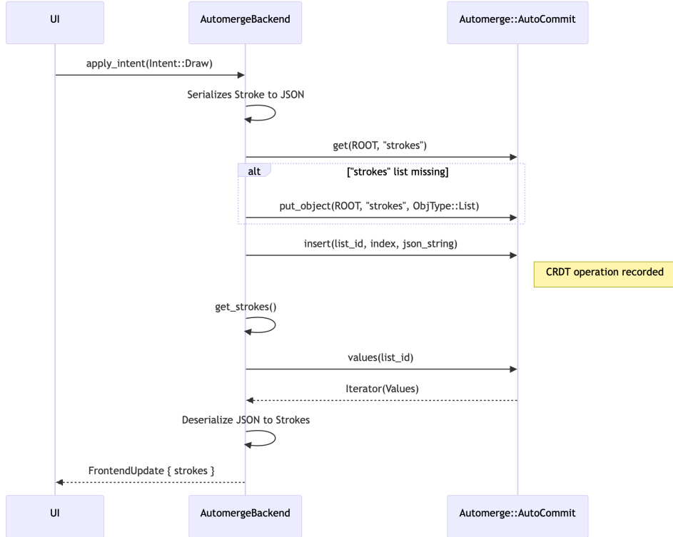
Figure 2.6: Sequence diagram of a local Intent::Draw operation
