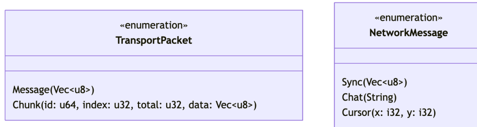
Figure 2.8: Transport and application-level message types: TransportPacket and NetworkMessage
